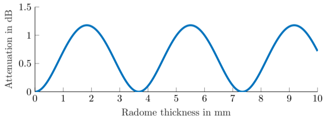
(b) Absorption values in dependency of the thickness of the radome material.
