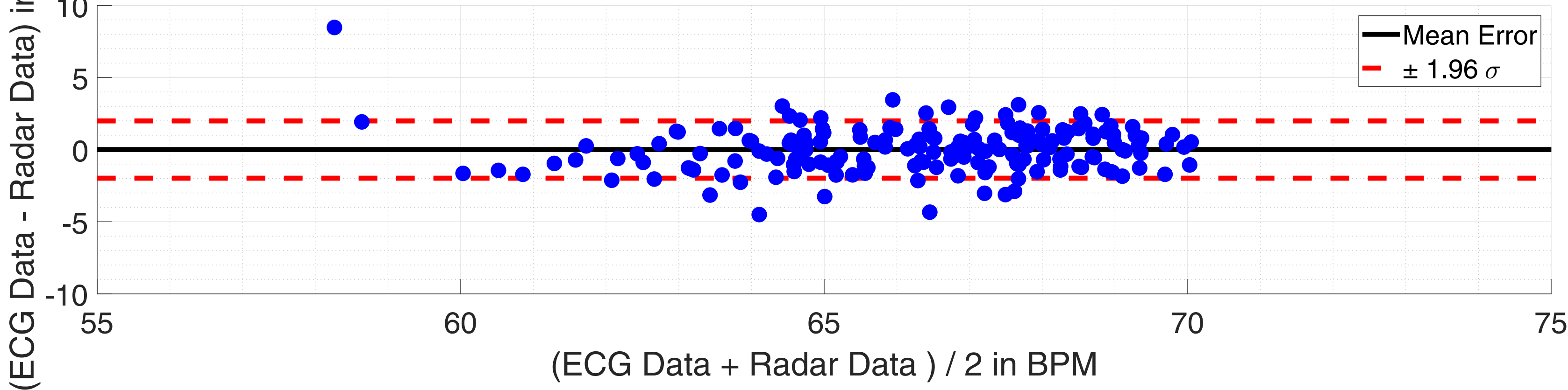
(b) Bland-Altman Plot for ECG vs Radar
