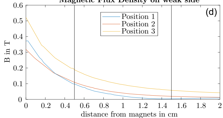
Magnetic Flux Density on weak side
