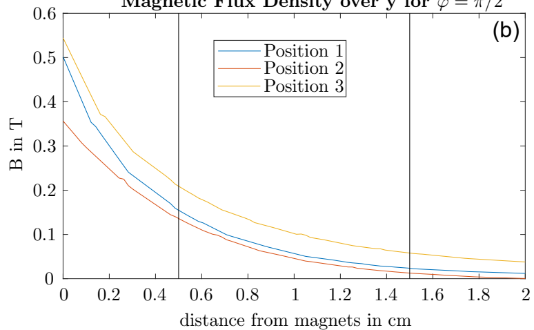
Magnetic Flux Density over y for \varphi = \pi/2
