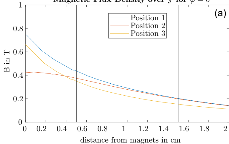
Magnetic Flux Density over y for \varphi = 0
