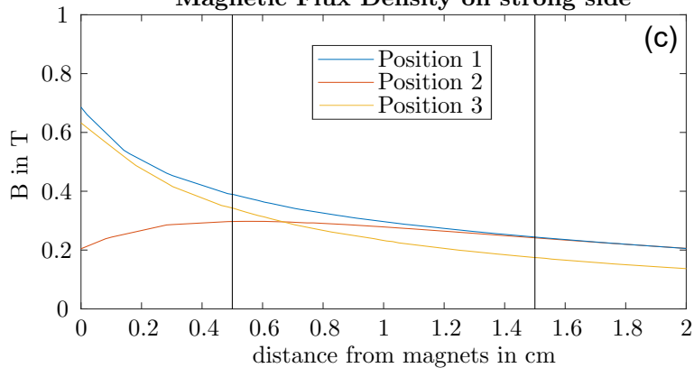
Magnetic Flux Density on strong side
